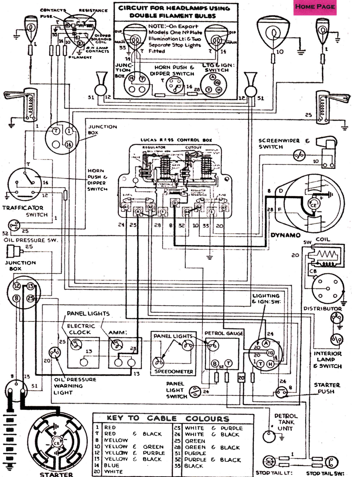
1950/51 CITROEN LIGHT 15 SALOON
