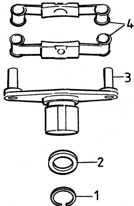
Fig. 2 Items fitted behind points box (Courtesy of Haynes Publishing)
