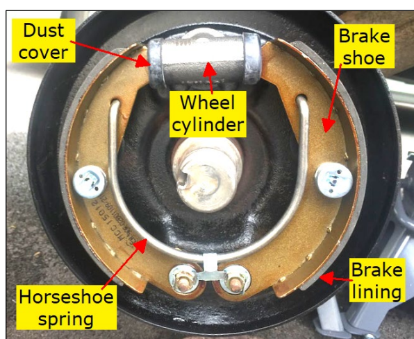
Fig. 2-15 Rear Brakes
