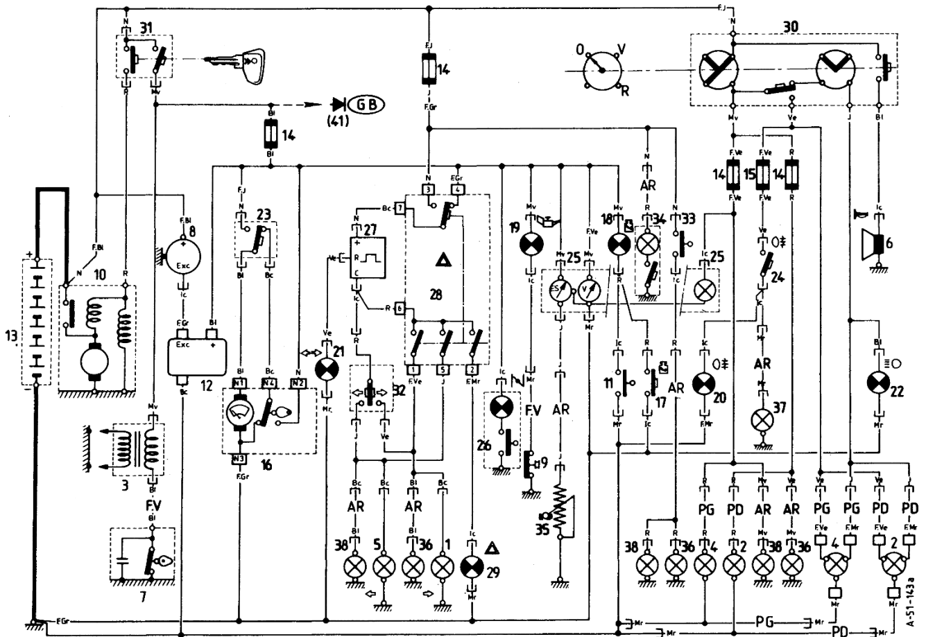
Fig. 4-5 1987 Standard 2CV Electrical Wiring Diagram (From Haynes Manual (1990), page 198)
